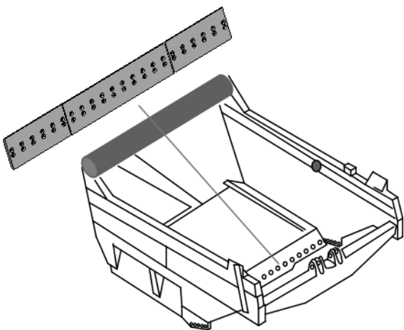
END EDGES CUCHILLA LATERAL
